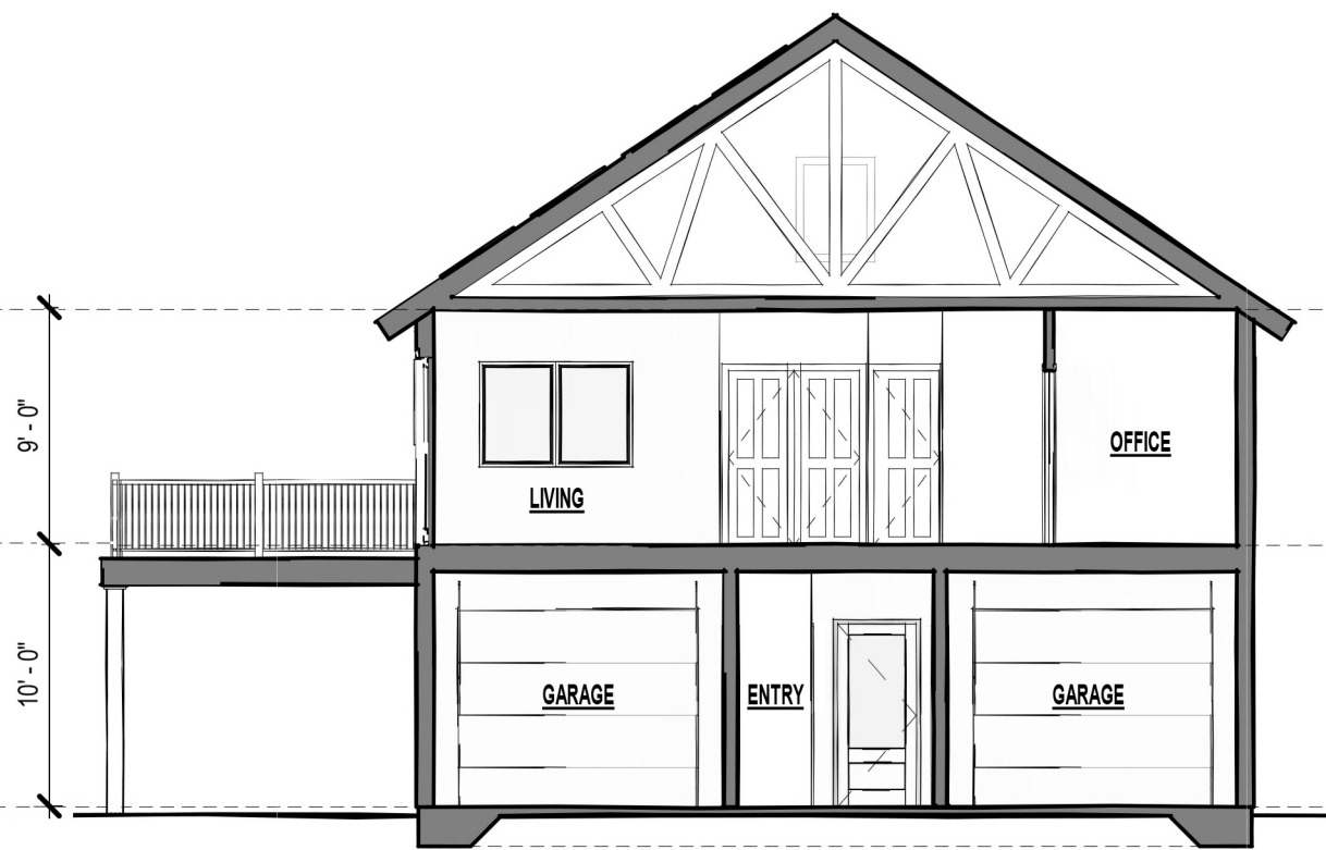
4 Cross Section 1/8" = 1'-0"
