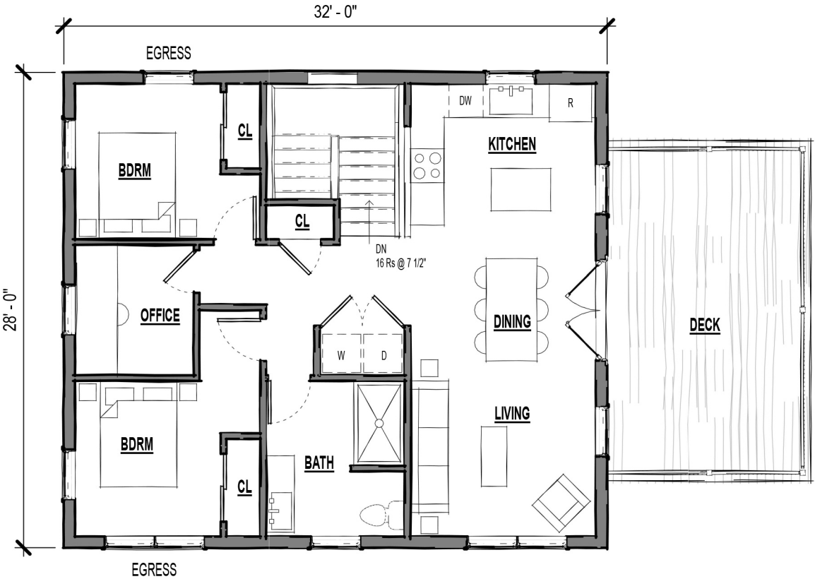
2 Second Floor Plan 1/8" = 1'-0"
