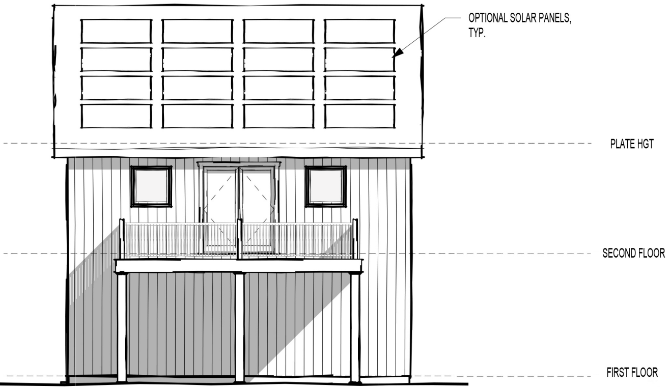
3 South Elevation 1/8" = 1'-0"
