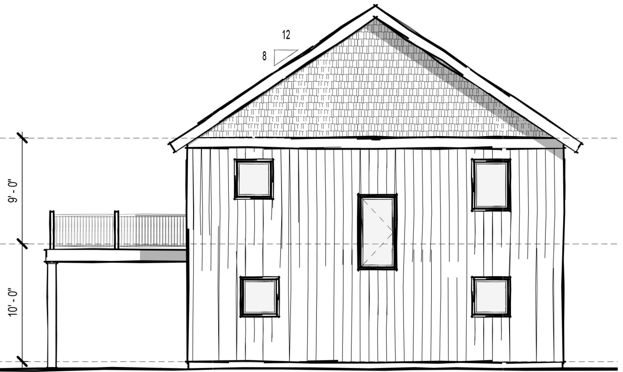
2 East Elevation 1/8" = 1'-0"
